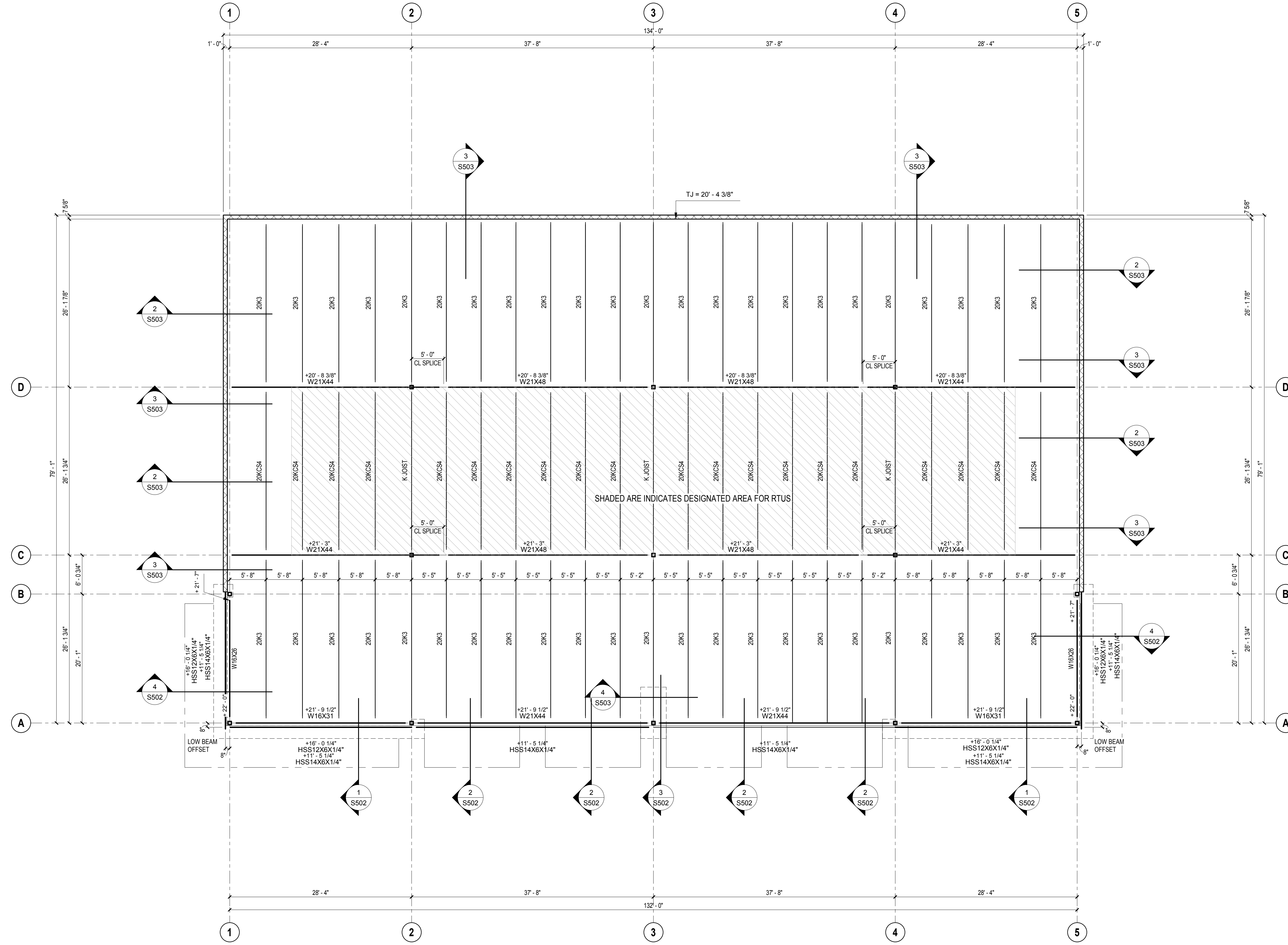
1 ROOF FRAMING PLAN 1/8" = 1'-0"
